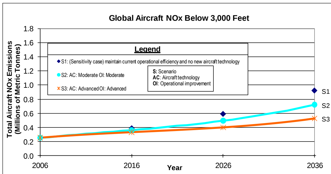
Figure 2. Total Global Aircraft NO x Below 3,000 Feet AGL.
