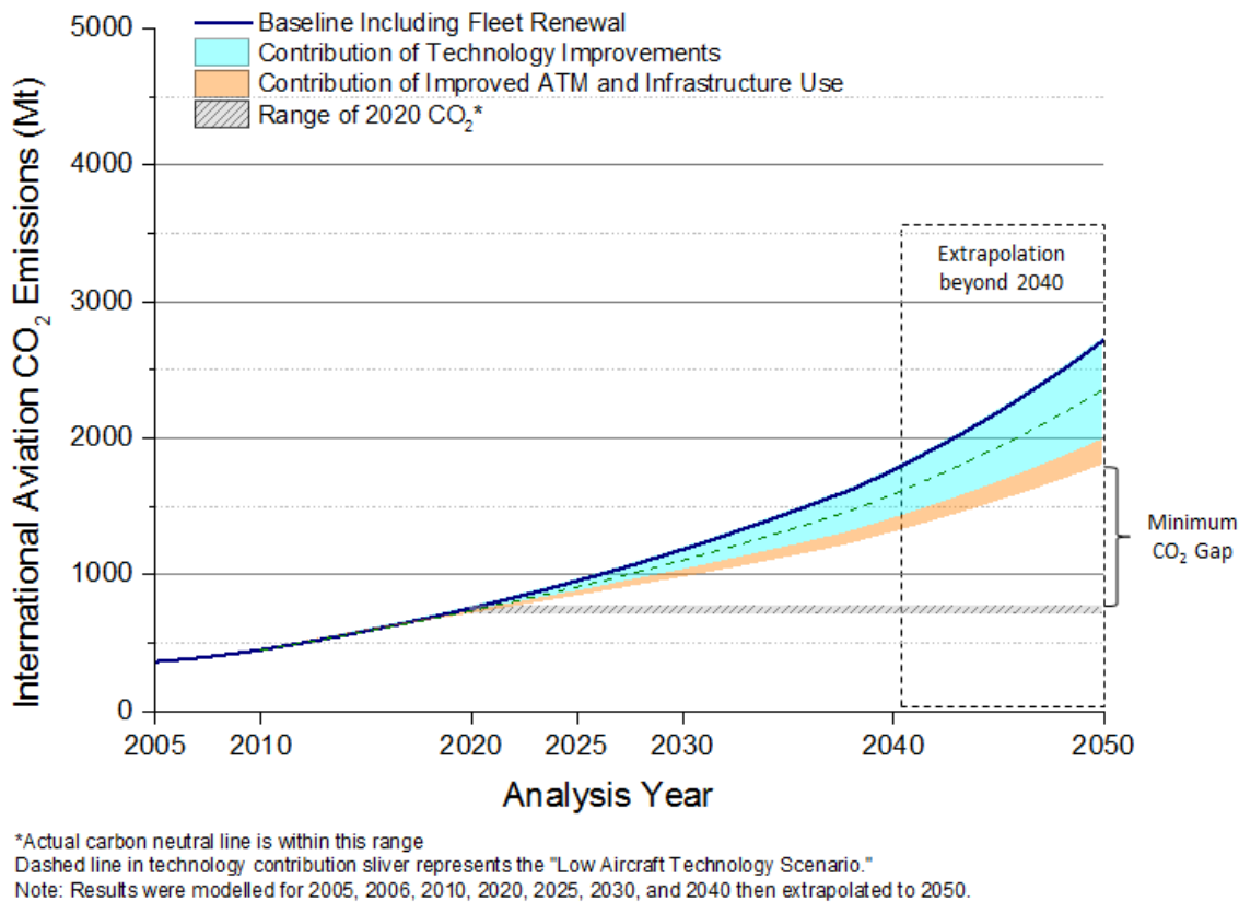
Figure 3. Aircraft CO 2 Emissions from International Aviation, 2005 to 2050.
