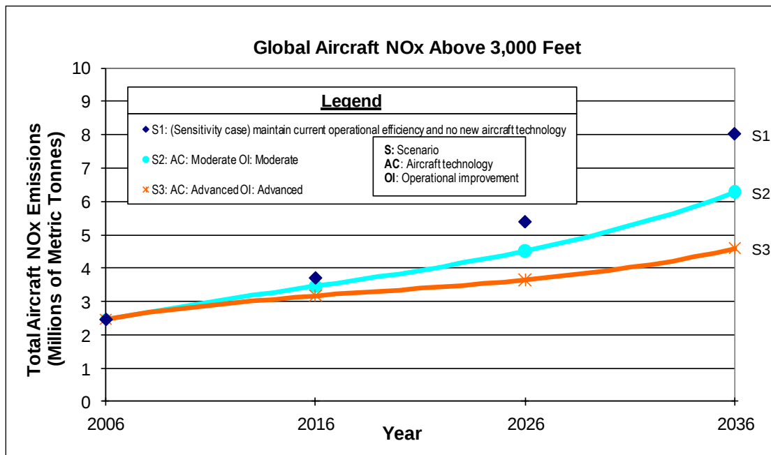
Figure 3. Total Global Aircraft NO x Above 3,000 Feet AGL.
