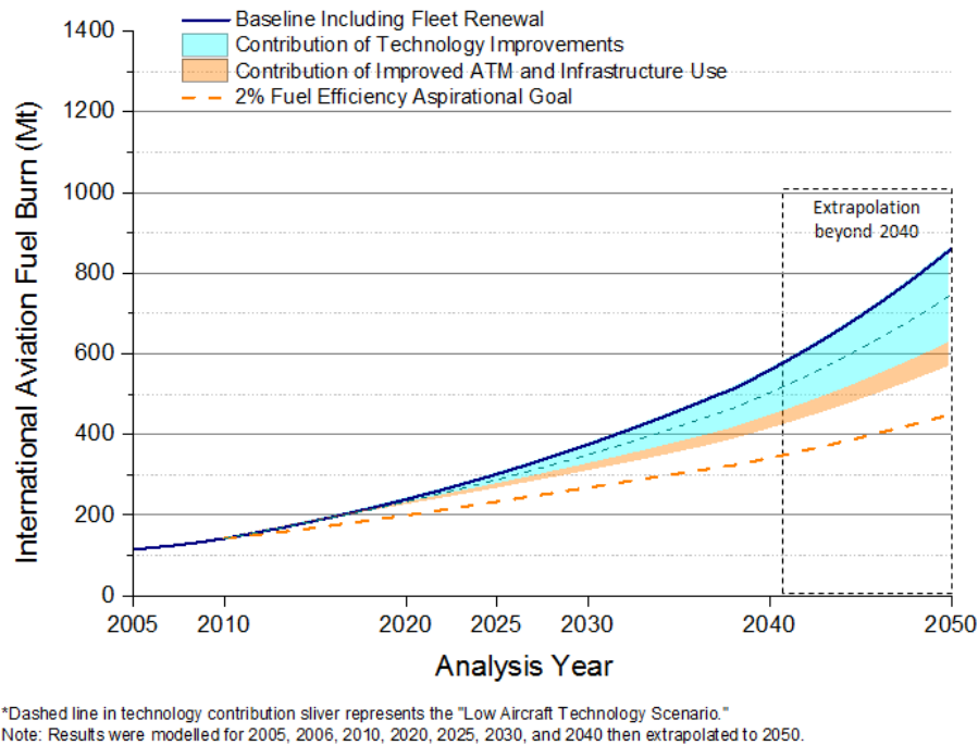
Figure 1. Aircraft Fuel Burn from International Aviation, 2005 to 2050.
