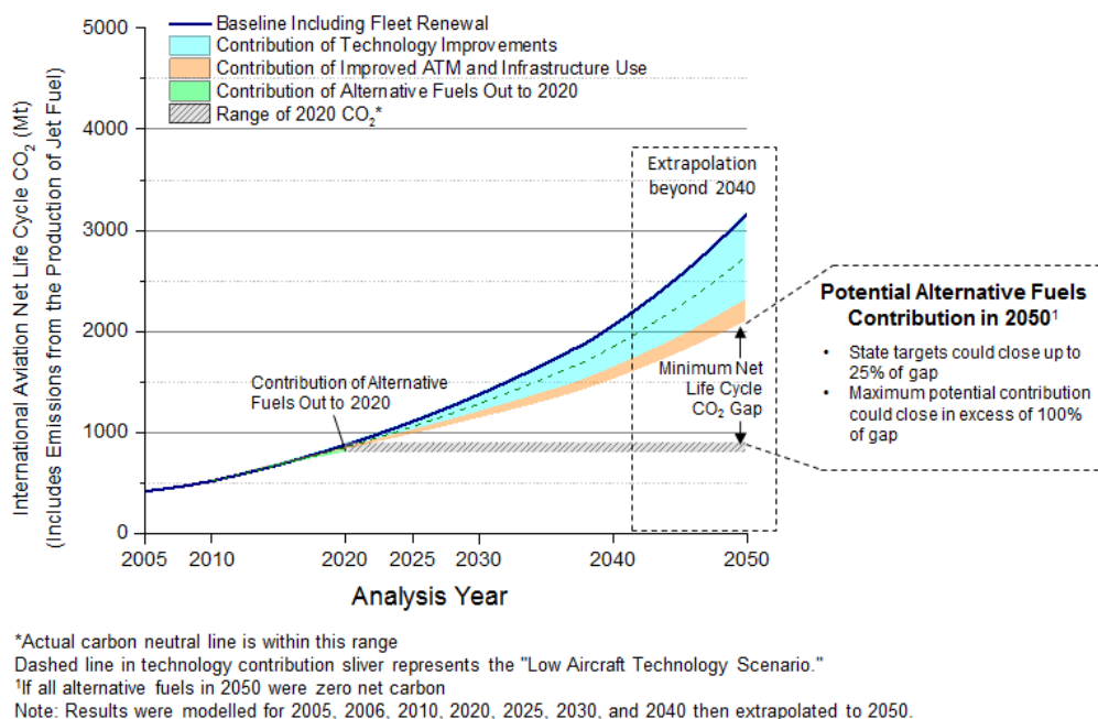
Figure 4: Contribution of Alternative Fuels Shown as International Aviation Net Life Cycle CO 2 Emissions, 2005 to 2050.
