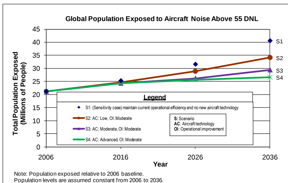
Figure 1. Total Global Population Exposed to Aircraft Noise Above 55 DNL.
